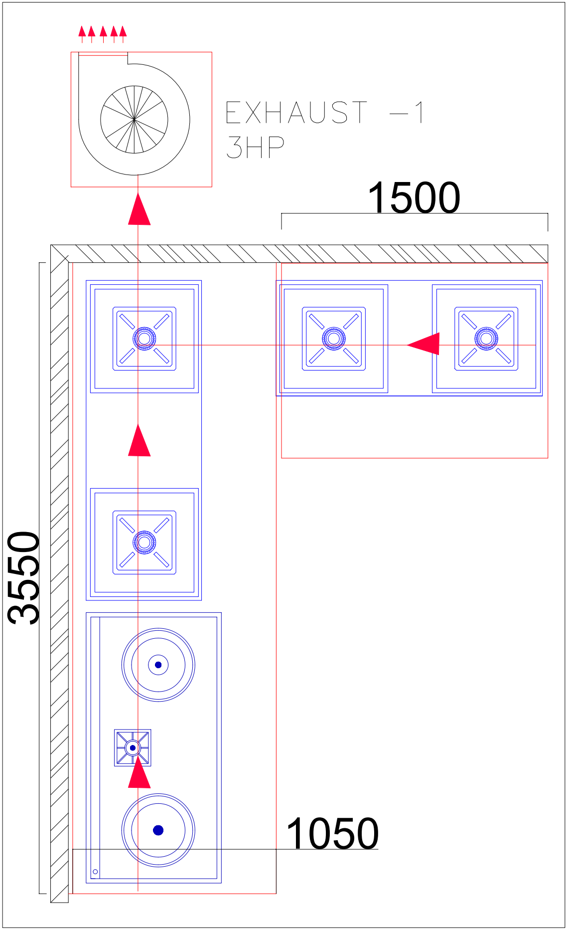
EXHAUST SYSTEM FOR BAGALUR RESTURANT
